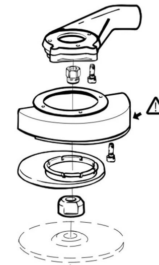
Spot suction kit for depressed center wheel
