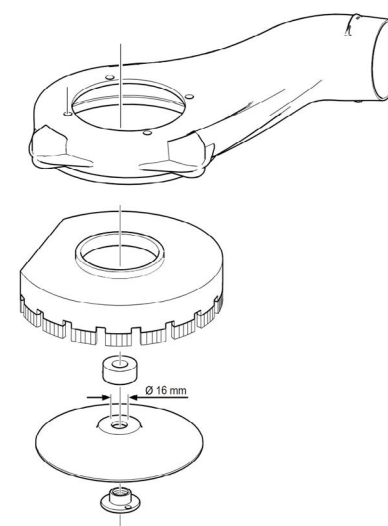
Spot suction kit for sanding with fibre disc
