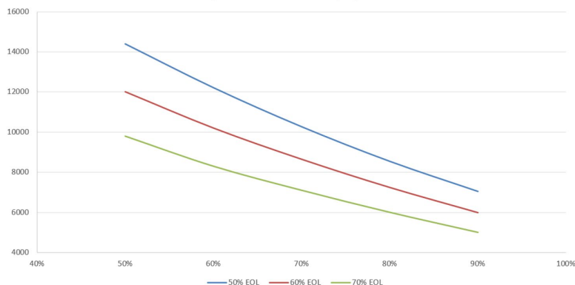
Cycle Life VS DOD @ varying EOL
