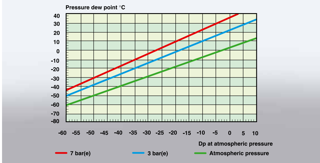
Relation between dew point and pressure dew point.
