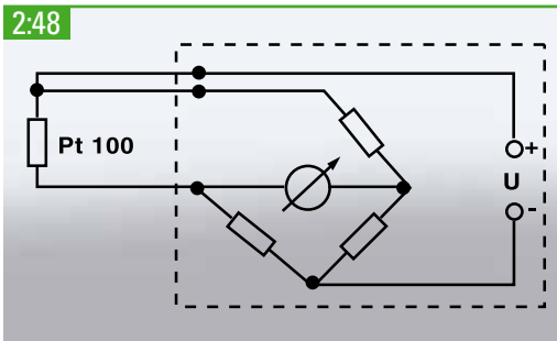
Example of a 3-wire connection using a resistance thermometer of 100 \Omega . The resistance thermometer and connectors are connected on a bridge.
