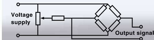
Bridge connection with strain gauges.
