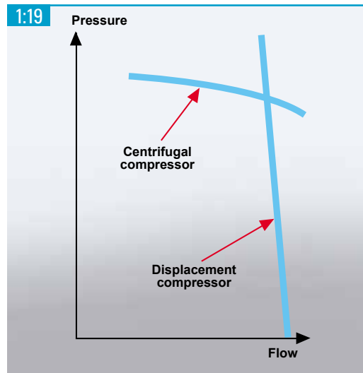
This illustrates the load curves for centrifugal respective displacement compressors when the load is changed at a constant speed.
