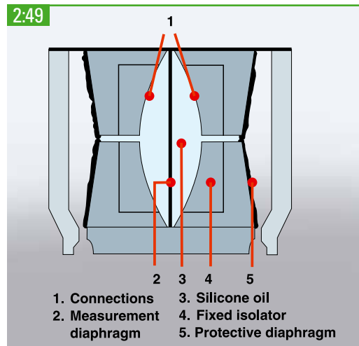
Example of a capacitive system for pressure measurement.
