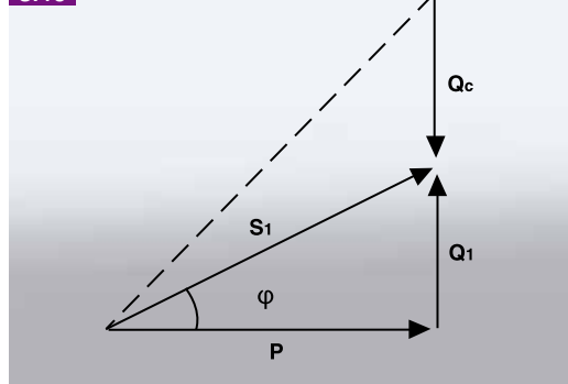
Reactive power Q_c is supplied to increase the motor power factor \cos(\varphi) to 1.
